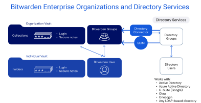
Bitwarden Enterprise Organizations and Directory Services Diagram
